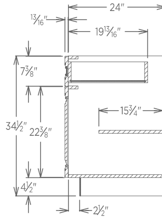
BASE CABINET
