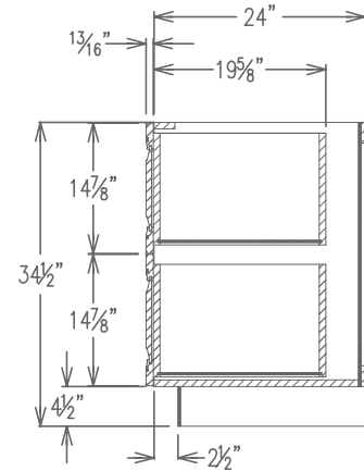
2-DRAWER BASE CABINET
